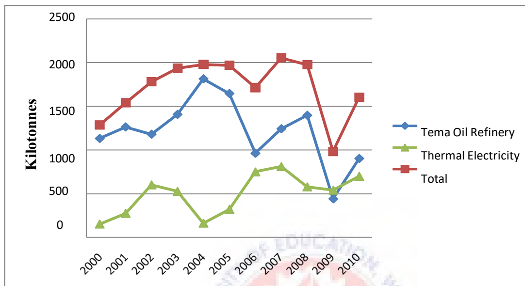
Figure 3: Trends of Petroleum Consumption by Power Thermal Plants and Oil Refinery (Energy Commission Ghana, 2010)
